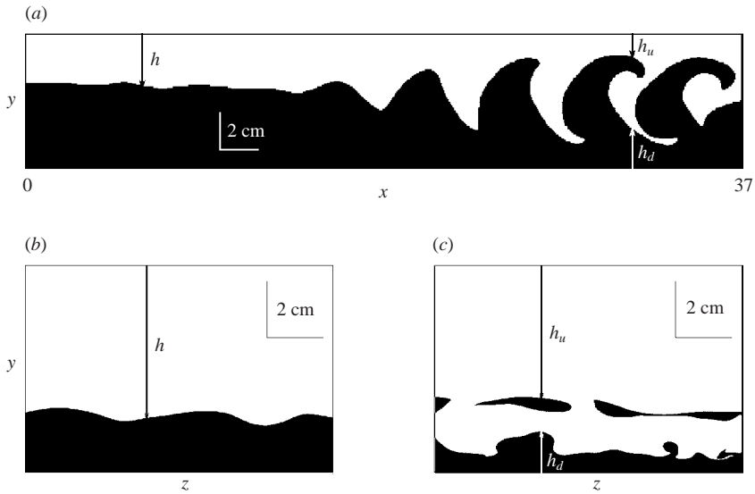
FIGURE 6. Interface elevation. Wake of a flat plate at Re_1 = 220 forced at the frequency f = 1.2 \text{ Hz} ( St = \delta f / \bar{U} = 0.07 ): (a) longitudinal section ( z = z_c , centre of the channel), (b) interface defined by a single line ( x = 6 \text{ cm} ), (c) folded interface ( x = 20 \text{ cm} ).
